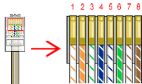
ETHERNET CABLE: RJ45 CONNECTOR
