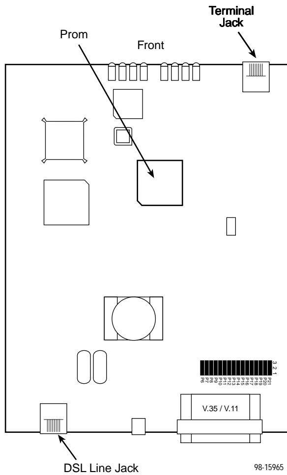
Figure 3. Model 7915 E1 Standalone Termination Unit with V.35 Interface
