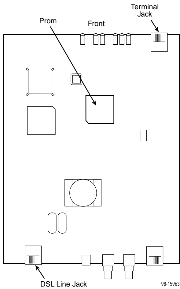
Figure 2. Model 7915 E1 Standalone Termination Unit with G.703 Interface
