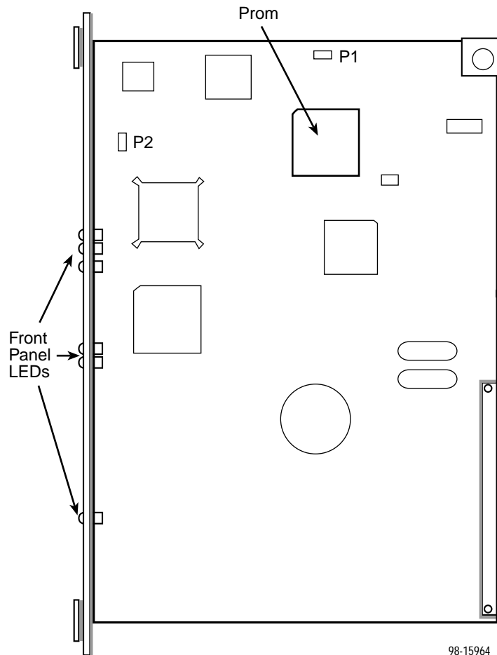
Figure 1. Model 7915 E1 G.703 Nest Card
